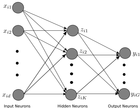
Figure : Graphical representation of Multi-Layer Perceptron (MLP).
