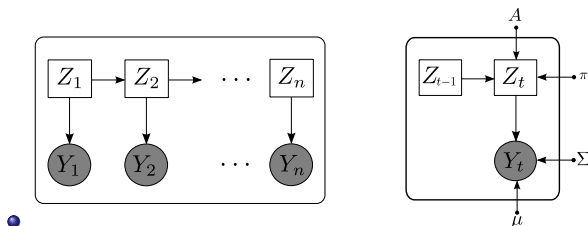
Figure : Graphical model structure for a Gaussian HMM.
